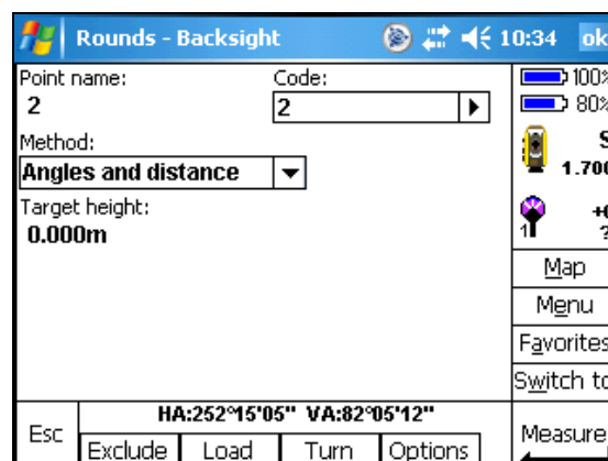
FIG 3. WHEN YOU HAVE A TARGET FILE AVAILABLE YOU CAN EASILY LOAD IT FOR A SECOND ROUND ON THE SAME SITE USING THE "LOAD" BUTTON WHEN YOU START A NEW ROUND.
