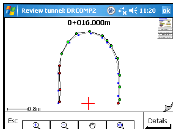
FIG 1. SCREEN SNAP OF THE TUNNEL REVIEW SHOWING POINTS OF OVER- AND UNCERCUT ON THE SCREEN OF THE CONTROLLER.
