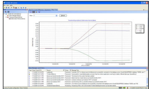
FIG 8. GRAPHICAL REPORT SHOWING DEFORMATION OVER TIME.
