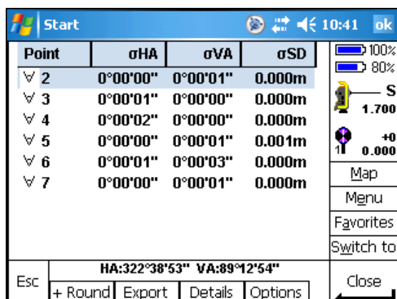
FIG 2. ONCE THE FIRST ROUND IS COMPLETED, YOU HAVE THE OPTION TO EXPORT THE TARGETS TO A TARGET FILE USING THE "EXPORT" SOFT BUTTON AT THE BOTTOM OF THE SCREEN
