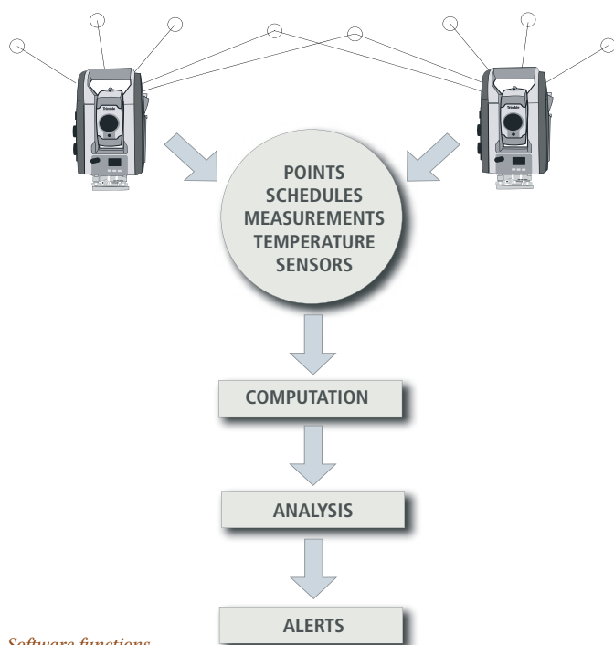
Software functions
